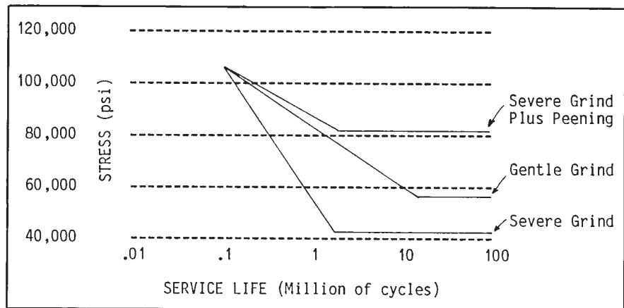
Fig. 1. Representative increase in resistance to cyclical loading produced by peening.
