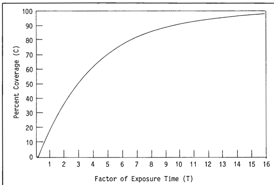
Fig. 2. Coverage versus exposure time.
