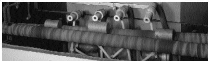
To eliminate the need for special fixtures and assure complete blast coverage, Empire developed a skew-roller conveyor for use in the customer's automated, in-line production process.
